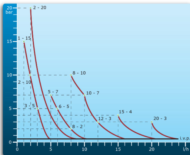
Pressione (bar) – Portata (l/h) Pressure (bar) – Flow Rate (l/h) Chart
